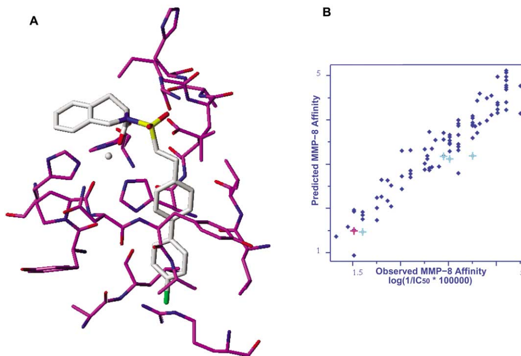
Figure 3. (A) Postulated binding mode of compound 96 within MMP-8 binding site. Only selected amino acid residues are shown. (B) Observed versus predicted MMP-8 affinities for utilized CoMFA model 19 with crossvalidated r^2 value of 0.569 for five components. Compounds used to derive this model are indicated by diamonds, while predictions for five new candidates are indicated by crosses.
