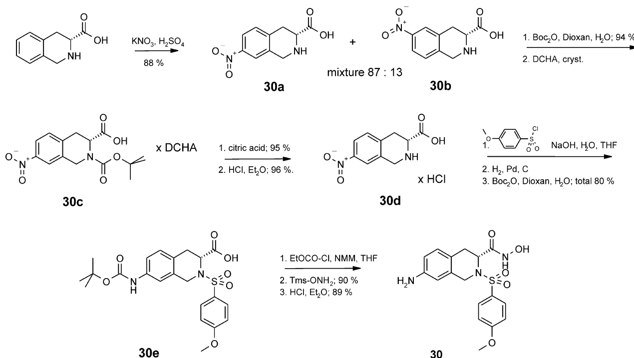
Scheme 3. Synthesis of nitro and amino-3-Tic derivatives.
