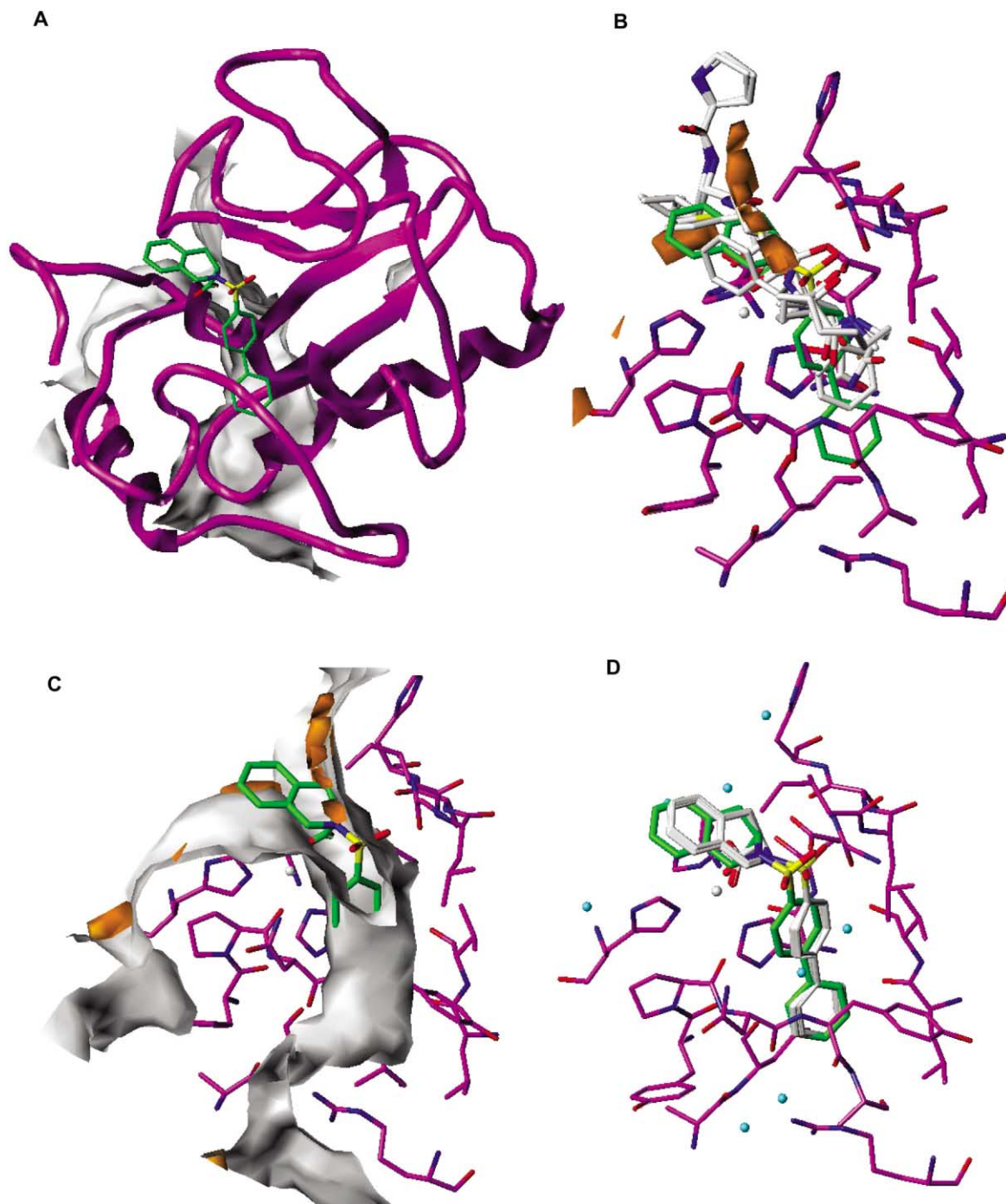
Figure 2. (A) Human neutrophil collagenase (MMP-8) fold from a 1.7 Å X-ray structure of the MMP-8/ 62 complex, 19 indicated by a magenta ribbon-tube encoding secondary structure elements, while compound 62 is displayed with green carbons. The MMP-8 inhibitor binding site is highlighted by a GRID 22 interaction energy contour map based on a methyl probe, drawn at +1 kcal/mol. Depth cueing is used to allow for a view into S1', where the biphenyl substituent is located. Similar models were obtained for public domain inhibitor complexes, serving as basis for our design. (B) Detailed MMP-8 binding site containing compound 62 with green carbons in comparison to public domain inhibitors from PDB files 1jan , 1jao , 1jap , 1jaq , 1mnc , 1kbc , 1mmb , 13 shown with grey carbons. Magenta carbons indicate selected protein residues from the above X-ray structure. Grey spheres indicate structurally conserved zinc ions. The MMP-8 binding site is highlighted by a GRID interaction energy contour (+1 kcal/mol) using a methyl probe, while hydrophobic regions are indicated by orange contours at −0.3 kcal/mol. (C) Detailed MMP-8 binding site containing compound 62 with green carbons. Regions with favourable hydrophobic interactions are indicated with orange contours at −0.3 kcal/mol from GRID interaction energies using a hydrophobic (DRY) probe. (D) 1.7 Å X-ray structure 19 of the MMP-8/ 62 complex (green carbons) compared to 10 best docking modes using FlexiDock (white carbons) after manual placement of a template in the MMP-8 cavity. Similar docking modes were used as basis for inhibitor design.
