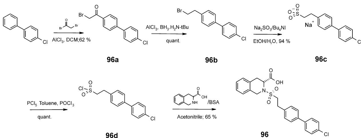
Scheme 2. Synthesis of the chlorobiphenylethyl-sulfonylchloride building block.
