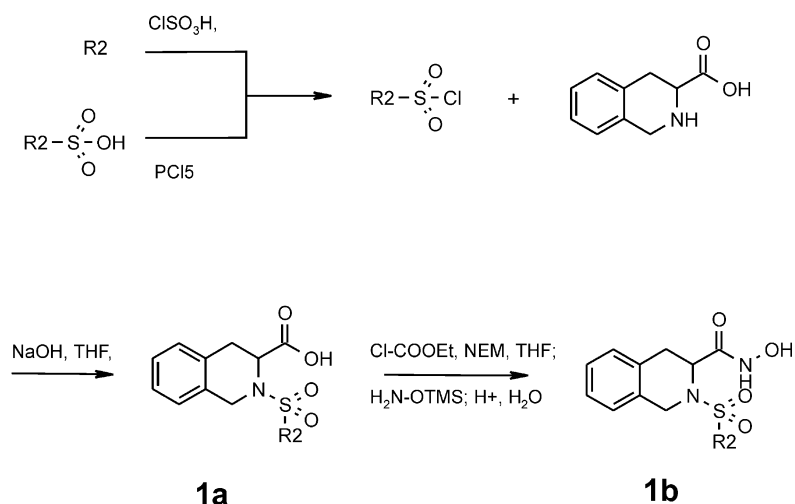
Scheme 1. Synthesis of 2-arylsulfonyl-1,2,3,4-tetrahydroisoquinoline-3-carboxylates and -hydroxamates.
