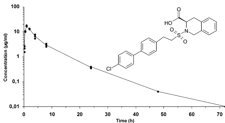
Figure 4. Mean concentration–time curve (µg/mL vs h) showing the plasma elimination profile of compound 96 . Administration of a single oral dose of 6 mg/kg in healthy beagle dogs ( n=2 ; vehicle: 1% CMC, 0.05% DONSS) gave a maximal plasma concentration C max of 17 µg/mL, with a half life of 7 h.
