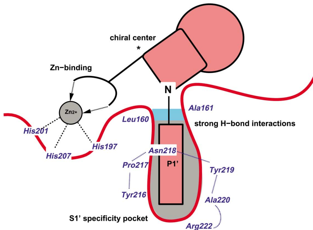
Figure 1. Schematic view to the MMP-8 binding site with key residues indicated. The bicyclic 1,2,3,4-tetrahydroisoquinoline scaffold provides ideal geometry to link S1' directed hydrophobic substituents with zinc complexing groups. Hydrogen bond acceptors are favourable at the S1' entrance, while the aromatic 1,2,3,4-tetrahydroisoquinoline ring is situated close to a hydrophobic region.
